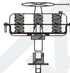
Manual and pneumatic clutch type actuator
