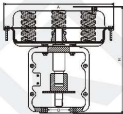
Pneumatic Diaphragm Actuator
